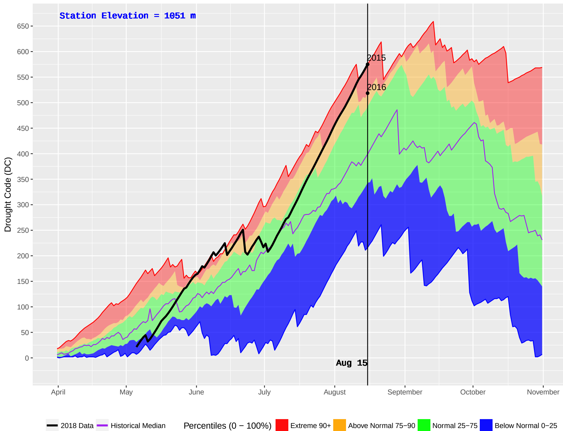
GOATHAVEN (886) : Historical (2005–2016) and Current (2018) Daily Drought Code (DC)
