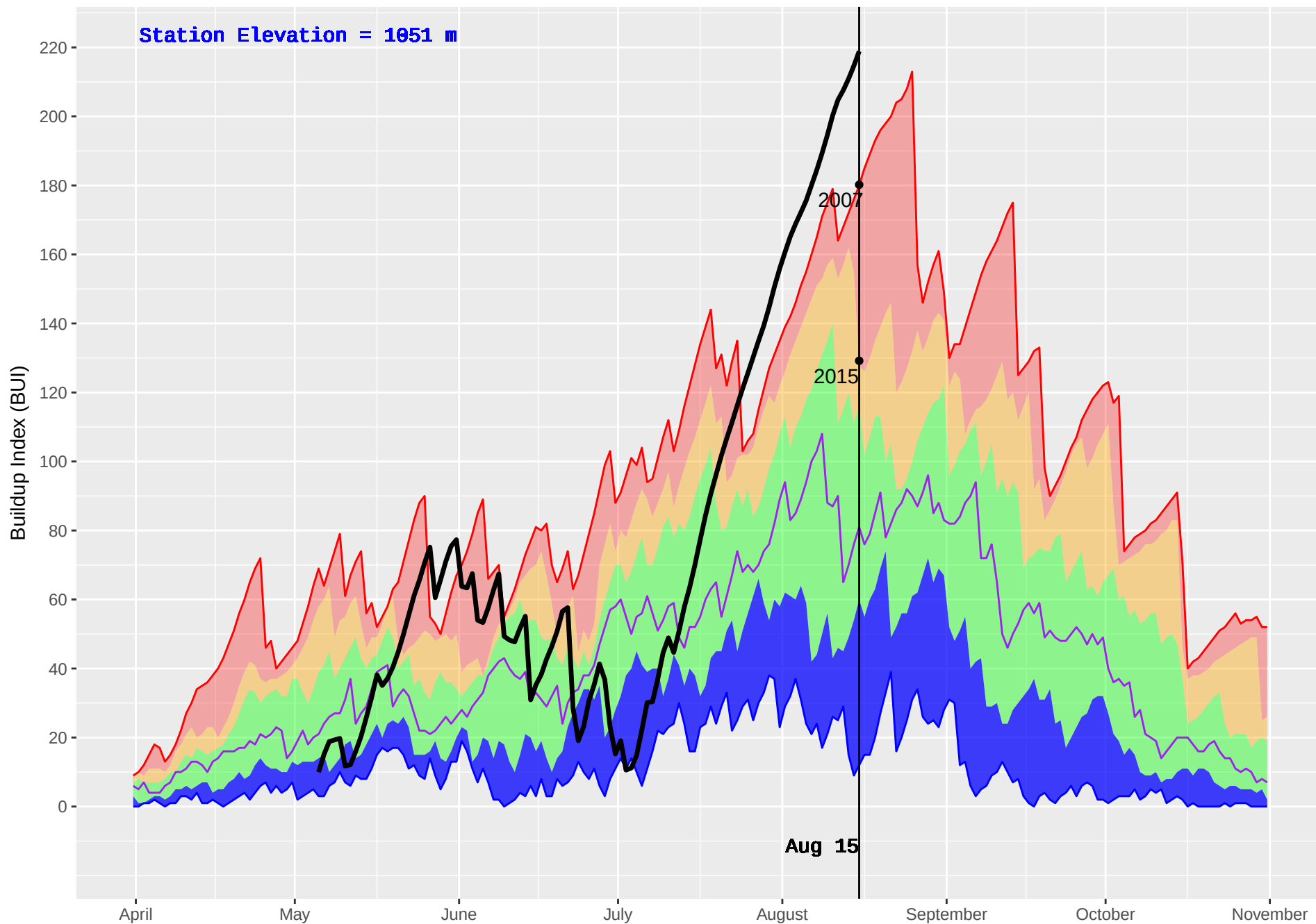
GOATHAVEN (886) : Historical (2005–2016) and Current (2018) Daily Buildup Index (BUI)
