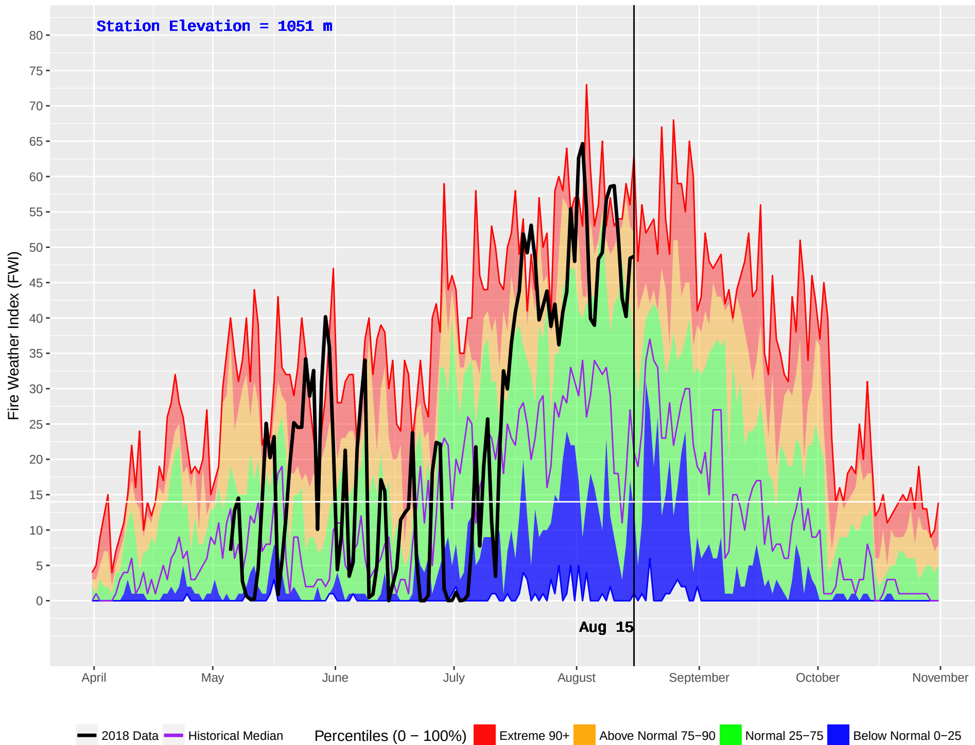
GOATHAVEN (886) : Historical (2005–2016) and Current (2018) Daily Fire Weather Index (FWI)
