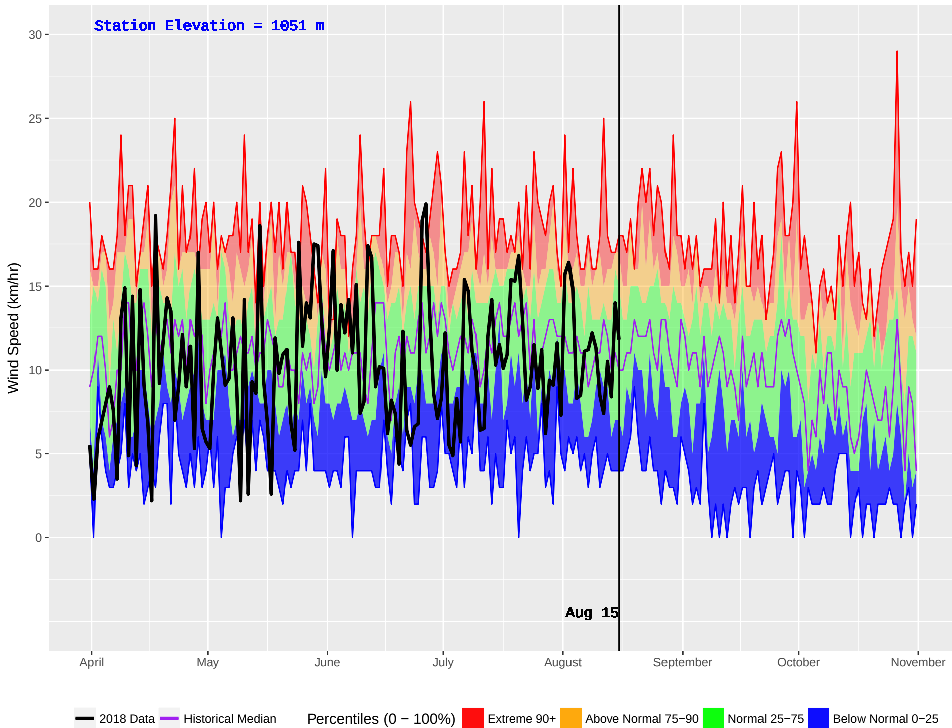
GOATHAVEN (886) : Historical (2005–2016) and Current (2018) Daily Wind Speed
