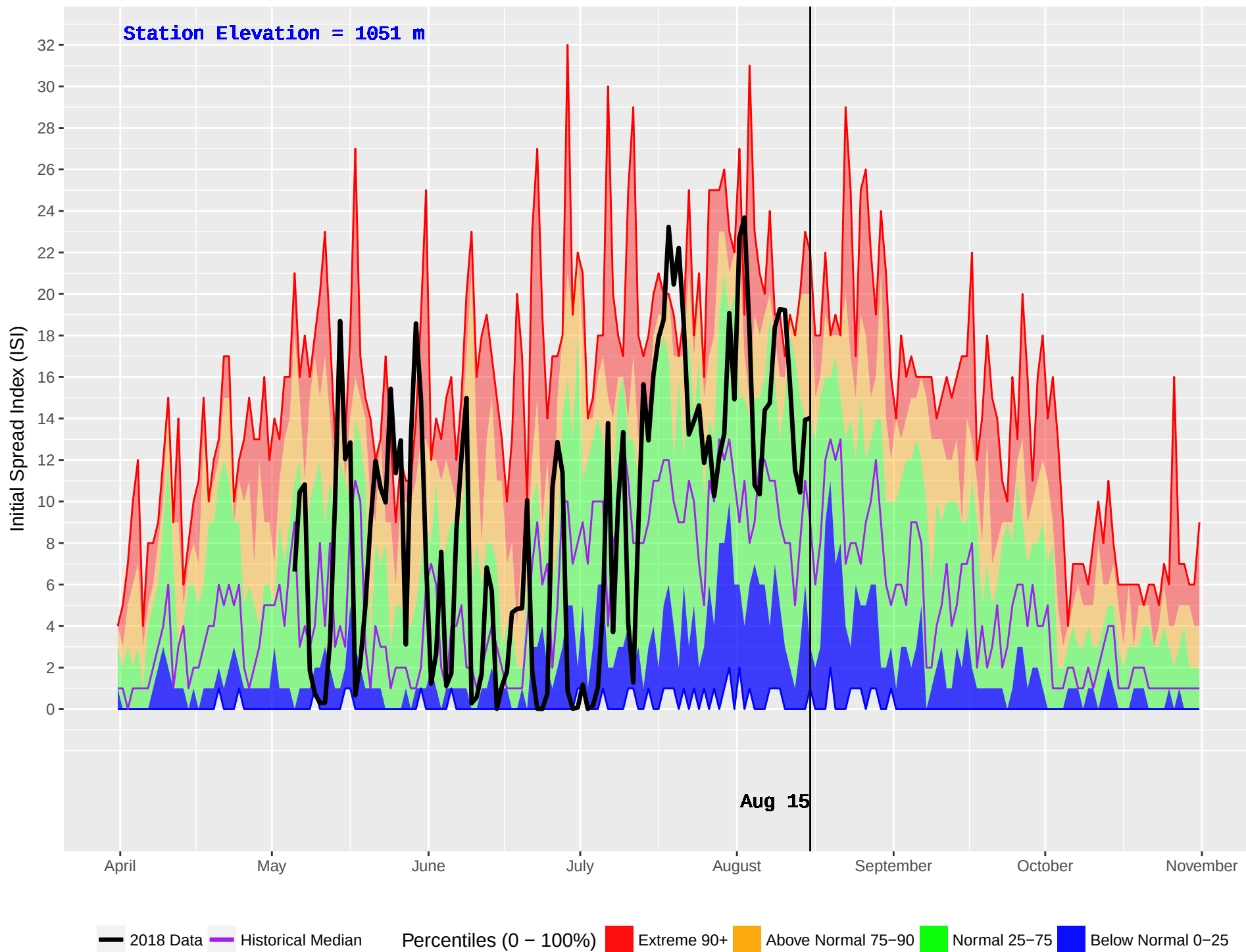
GOATHAVEN (886) : Historical (2005–2016) and Current (2018) Daily Initial Spread Index (ISI)
